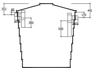
SECTION - SEPTIC
