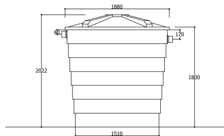
ELEVATION - SEPTIC
