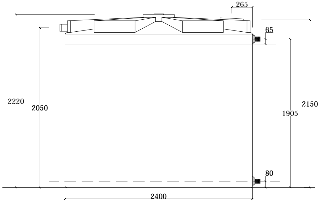
Elevation - 10K litre WT
